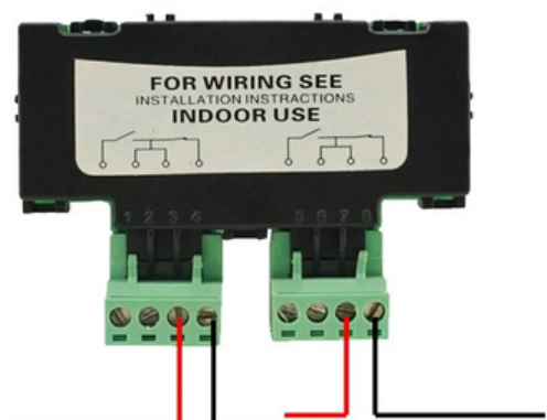
NC(Normal Close)
