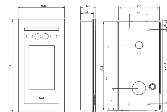
Flush-mount
