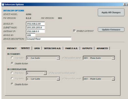
Fig. 20 Video Intercom - Service tab
