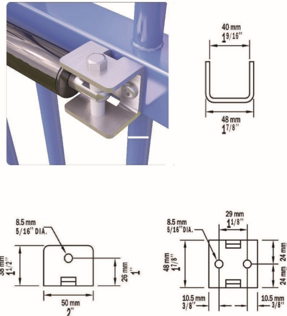
Gate Bracket
