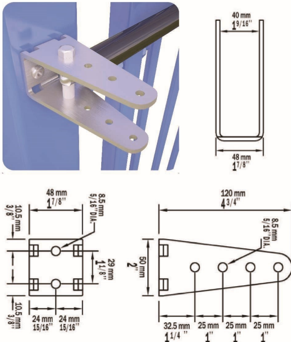
Post Bracket
