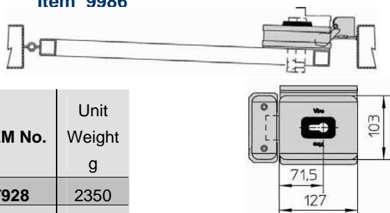
HORIZONTAL INSTALLATION
