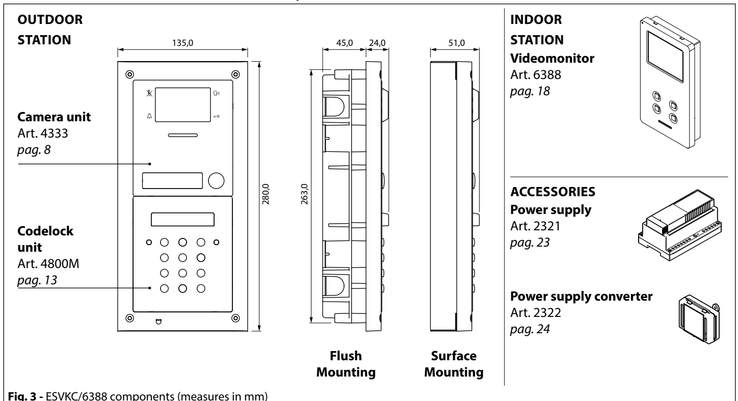
Fig. 3 - ESVKC/6388 components (measures in mm)
